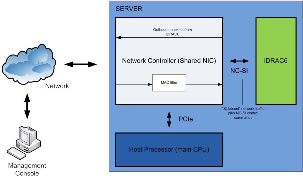
Figure 2 – NC-SI sideband interface
